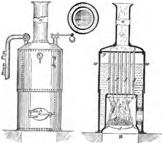
FIGS. 121, 122 and 123.—Exterior and sectional elevation of an upright stationary boiler, also plan, showing the grate bars and the surrounding waterleg. In these figures, A is the fuel feed door; a is the chimney; f, f, f, the flues; w, w, the water level; c, c, the lower tube plate; g, the upper tube plate. The feed water is heated in the waterleg around the fire box.
